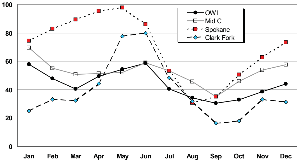
Figure 5.3: NW & Avista Monthly Hydro Capacity Factors Modeled in AURORA XMP (%)
