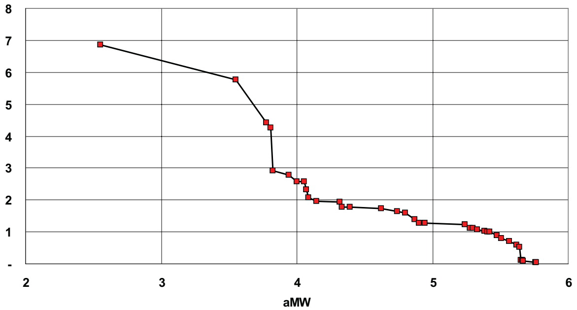
Figure 3.6 Conservation Supply Curve (TRC B/C Ratios < 10.0)
