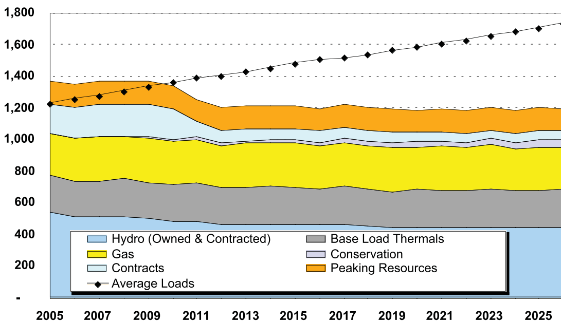
Figure 2.2: Energy Load and Resource Tabulation (aMW)
