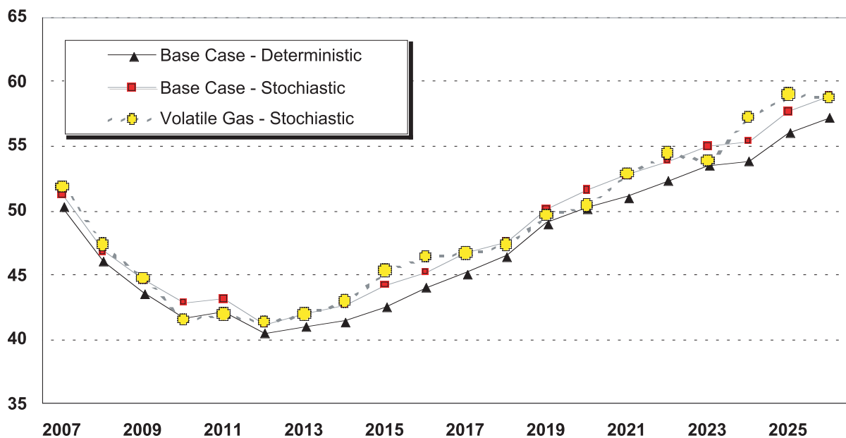
Figure 6.6: Mid-Columbia Electric Price Forecast Comparison ($/MWh)
