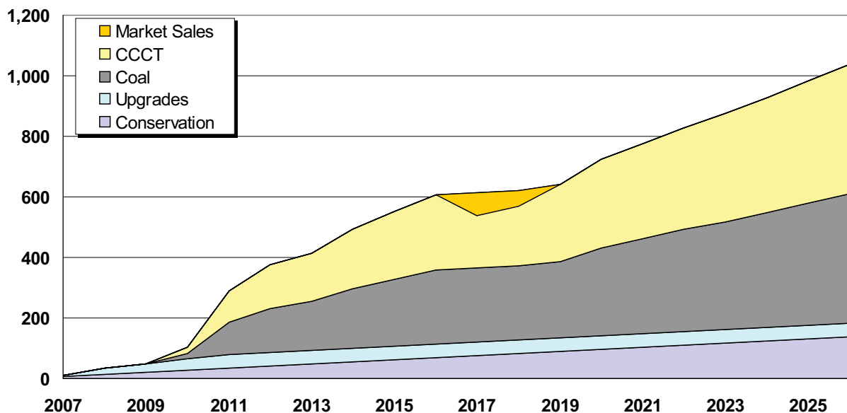
Figure 7.5: 50/50 Gas and Coal Build (MW)
