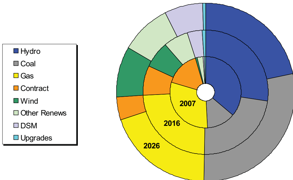
Figure 7.34: Company Resource Mixes (% of Energy) 2007, 2016, and 2026
