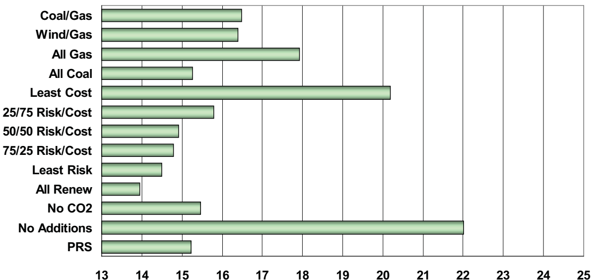
Figure 7.25: 2007-16 Power Supply Expense Average Covariance–Volatile Gas (%)
