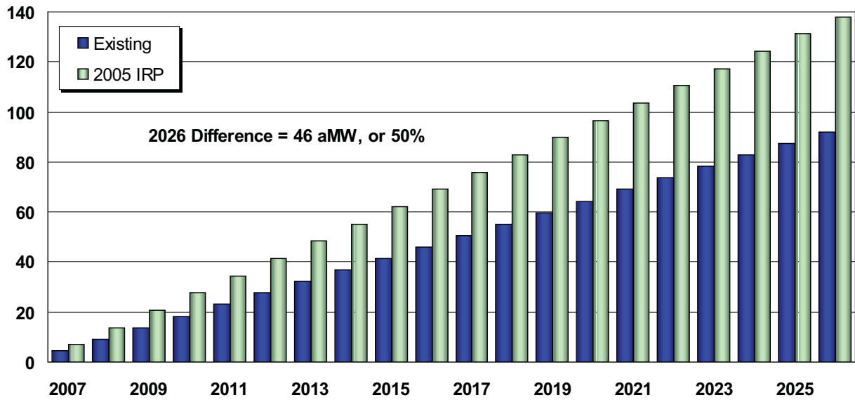
Figure 7.16: Conservation Acquisition (aMW)
