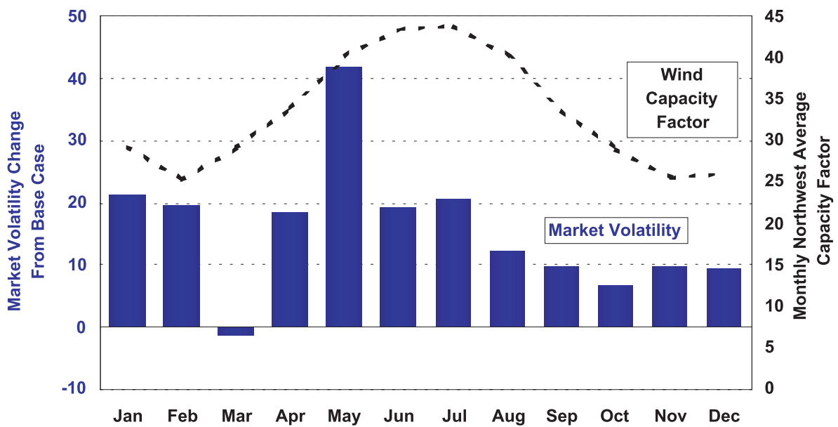
Figure 6.23: Monthly Market Price Volatility From Increased Wind Penetration (%)
