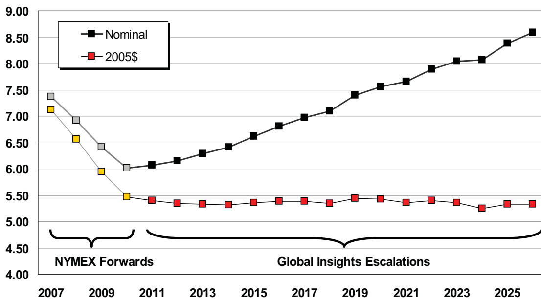
Figure 5.5: Henry Hub Natural Gas Price Forecast ($/dth)
