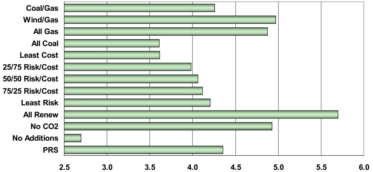
Figure 7.21: 2007-16 Average Incremental Power Supply Expense-Induced Rate Increases (%)
