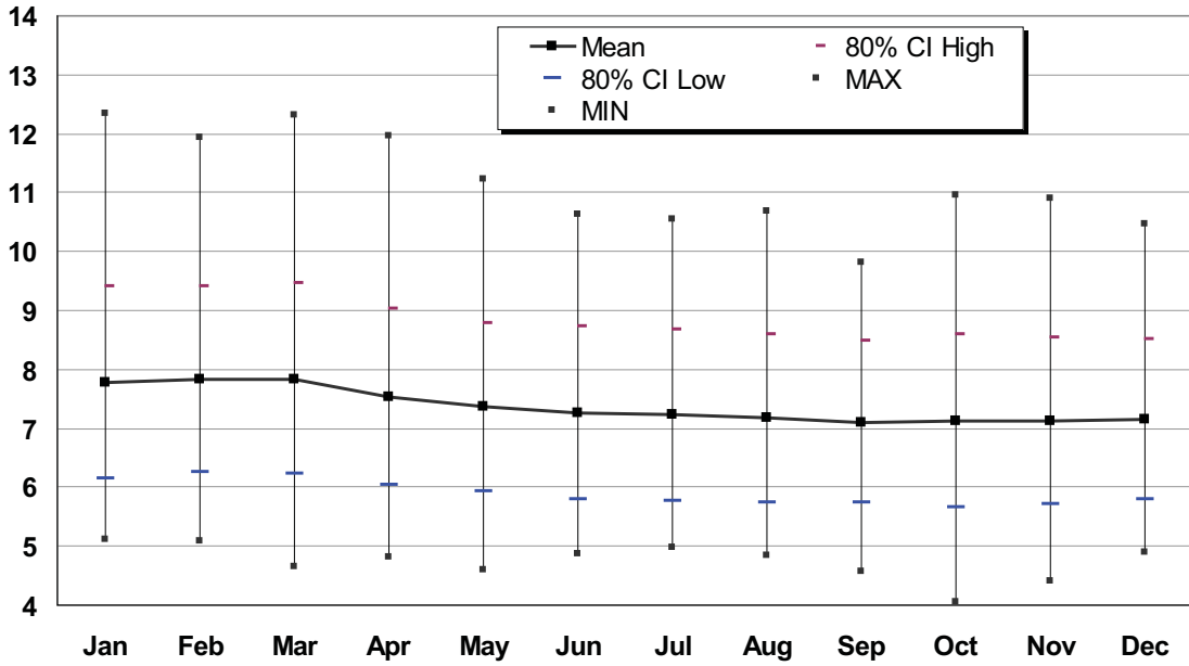
Figure 5.9: Natural Gas Price Statistics-2007 ($/dth)
