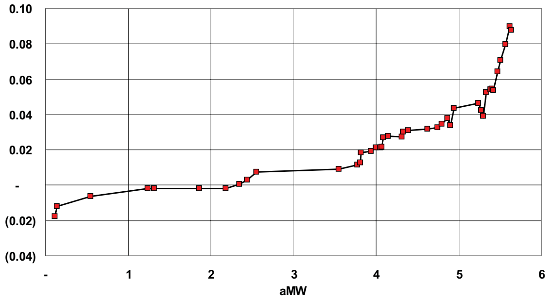
Figure 3.4: Conservation Supply Curve Stacked by Levelized TRC Cost <0.10 ($)
