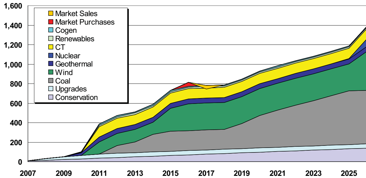
Figure 7.10: 25% Risk Build (MW)
