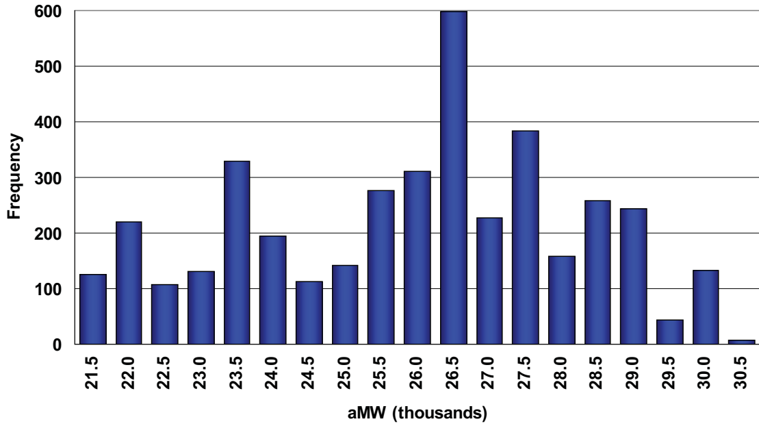
Figure 5.7: Western Interconnect Hydroelectric Generation Distribution
