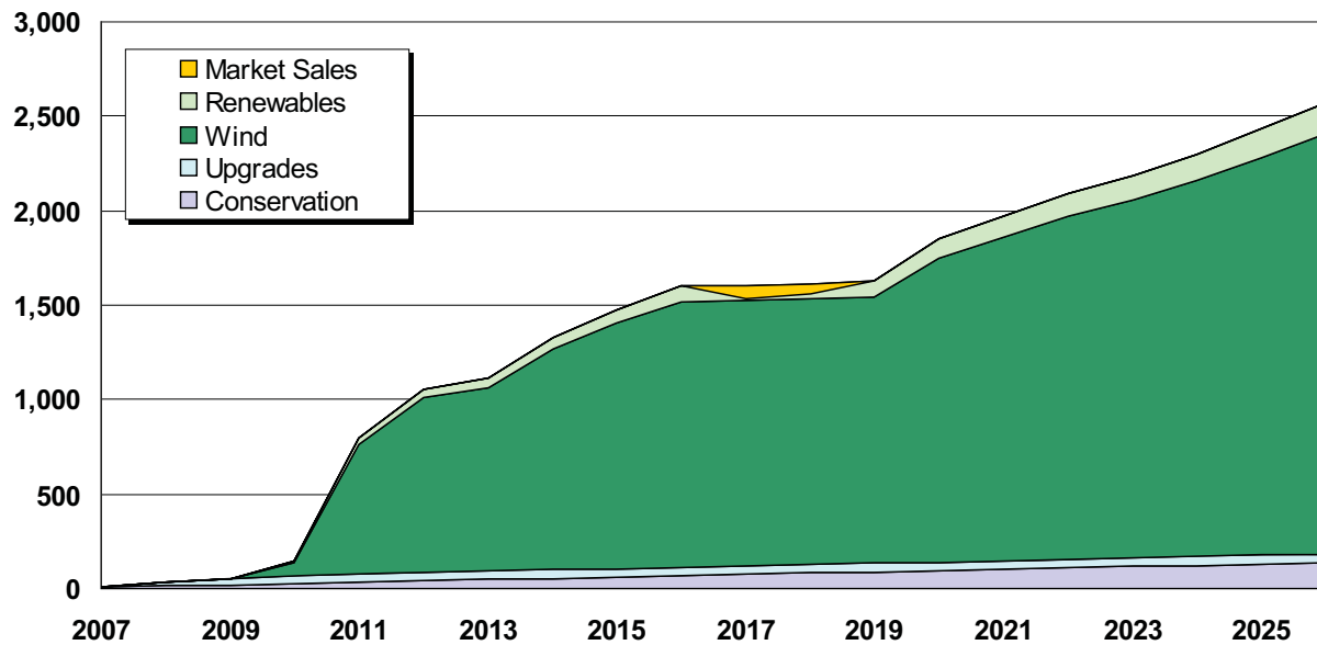
Figure 7.8: All Renewables Build (MW)
