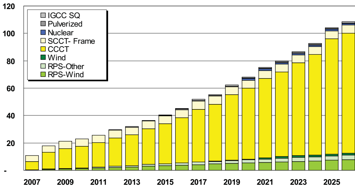
Figure 6.29: Cumulative Resource Selection for the Western Interconnect – NCEP Carbon Tax (GW)
