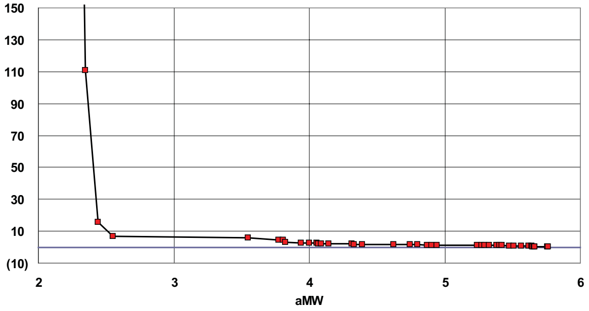
Figure 3.5: Conservation Supply Curve (TRC B/C Ratios)
