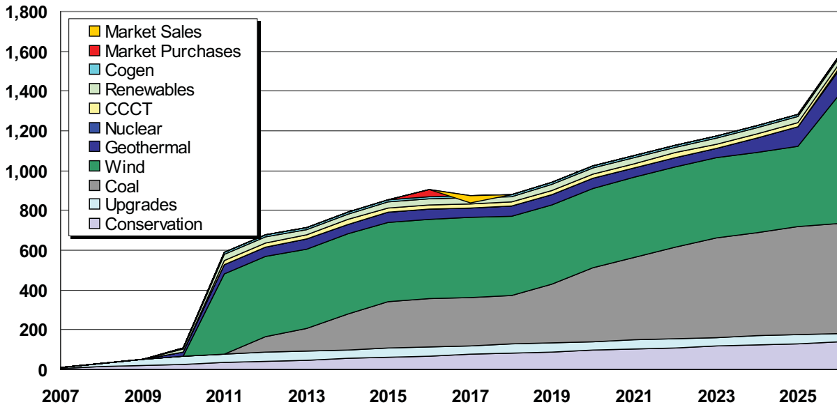
Figure 7.12: 75% Risk Build (MW)
