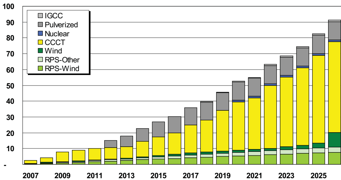
Figure 6.17: Cumulative Resource Selection for the Western Interconnect–No Capacity Credit (GW)
