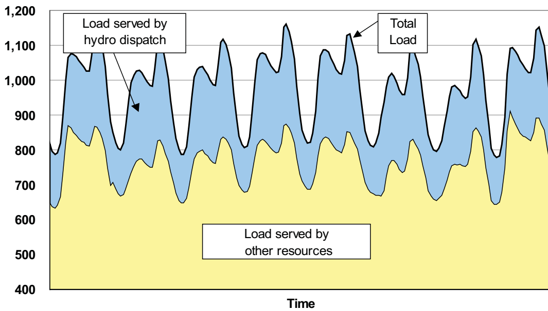
Figure 5.4: One Week Hydro Dispatch Example (MW)
