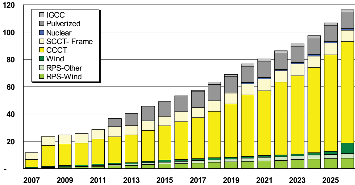
Figure 6.21: Cumulative Resource Selection for the Western Interconnect-Hydro Shift (GW)
