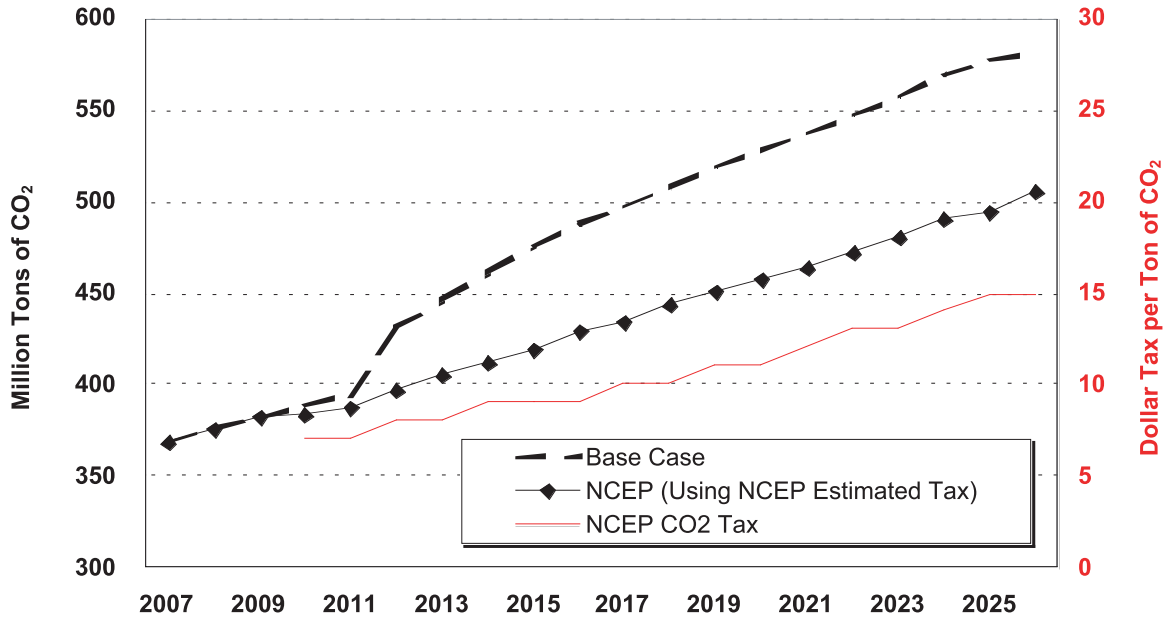
Figure 6.30: Western Interconnect Generator CO 2 Emissions Forecast
