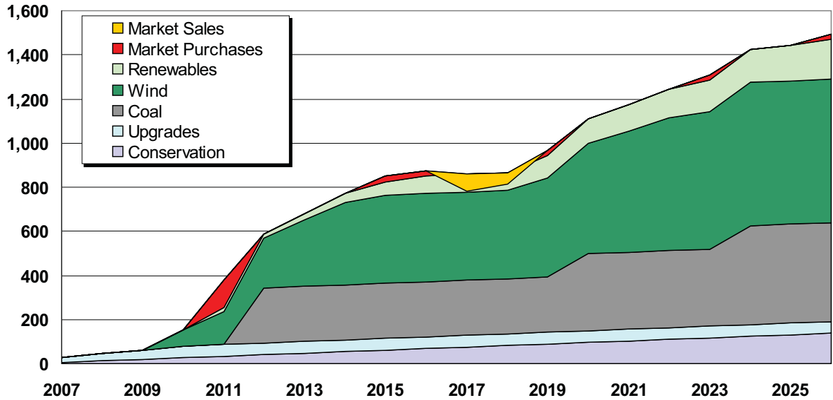
Figure 7.1: 2005 Preferred Resource Strategy Build (MW)
