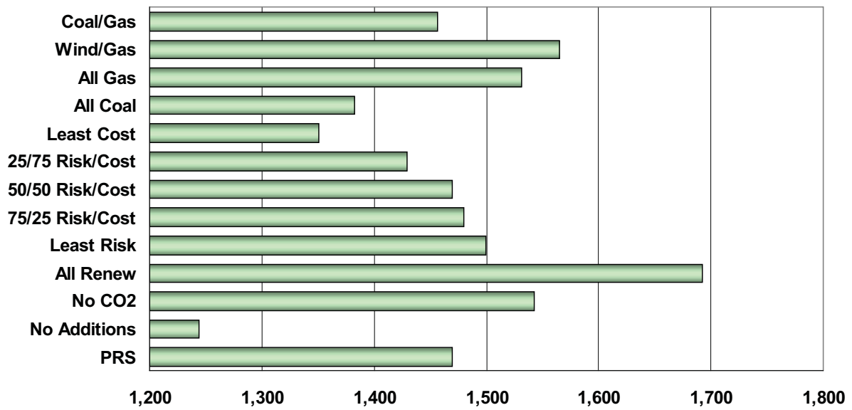
Figure 7.23: 2007-16 Incremental Power Supply Expense NPV ($millions)
