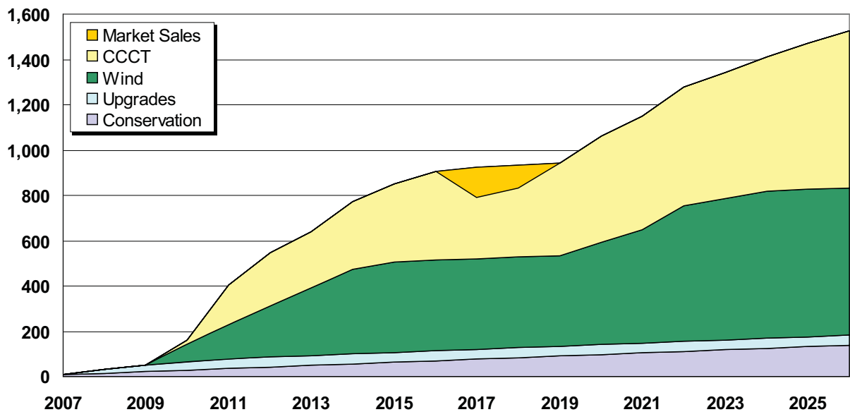
Figure 7.6: Wind and Gas Build (MW)
