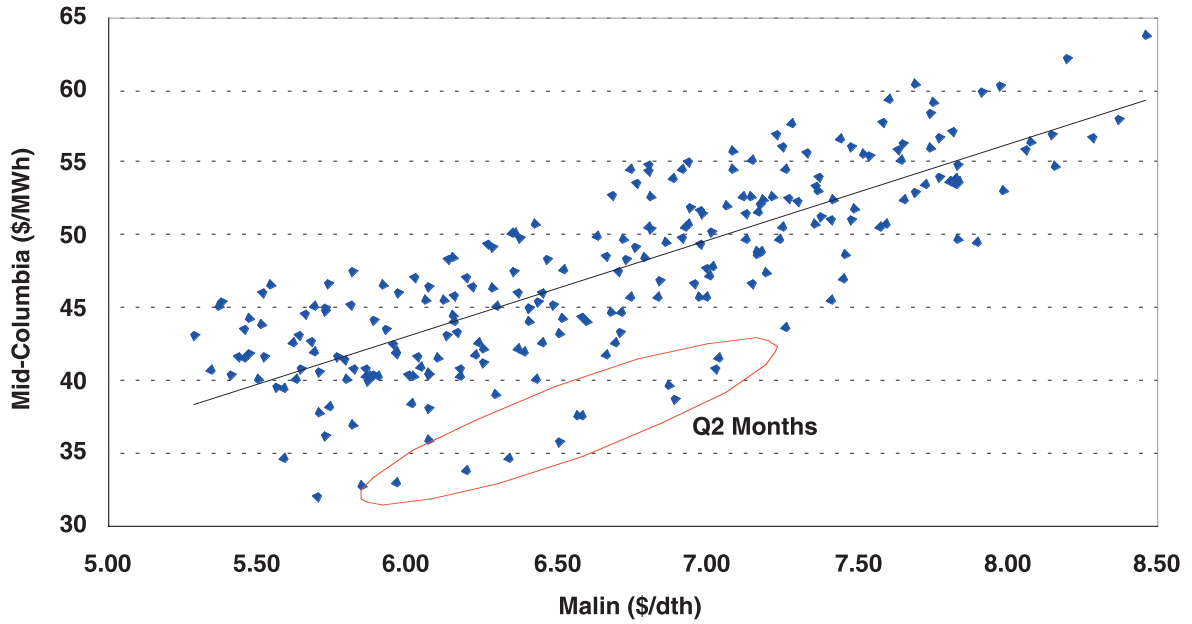
Figure 6.4: Malin Natural Gas and Mid-Columbia Electricity Correlation Plot
