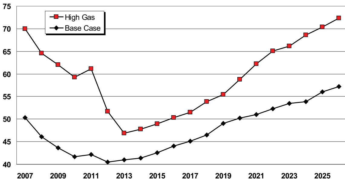
Figure 6.11: Base Case and High Gas Mid-Columbia Electric Price Forecasts ($/MWh)
