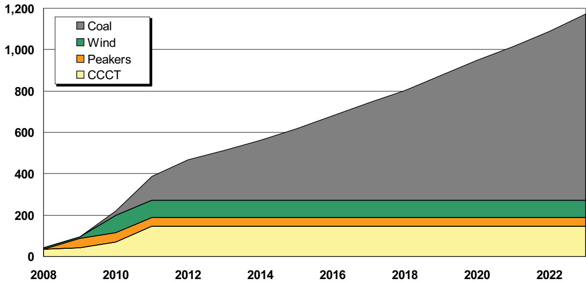
Figure 7.2: 2003 IRP Preferred Resource Strategy Build (MW)
