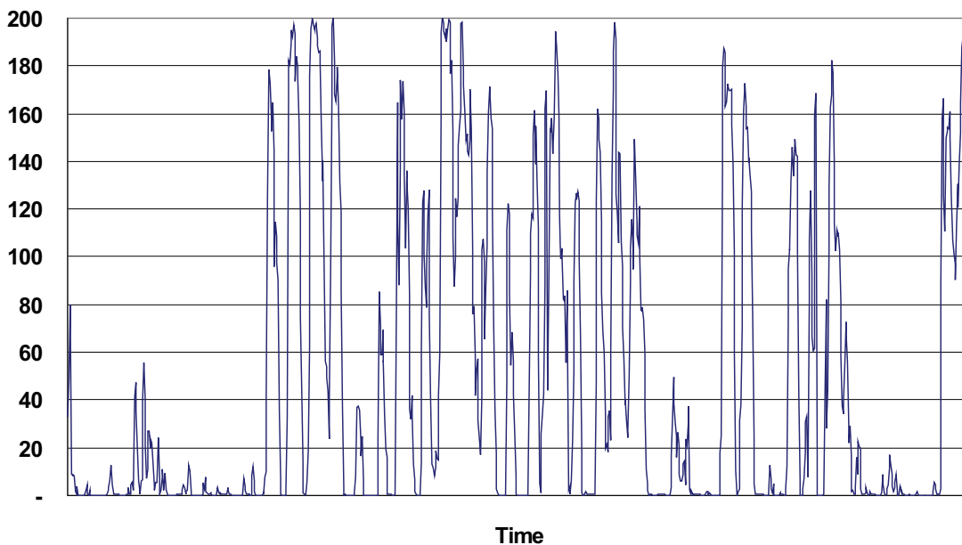
Figure 5.11: Actual Wind Data - 1000 Continuous Hours (aMW)
