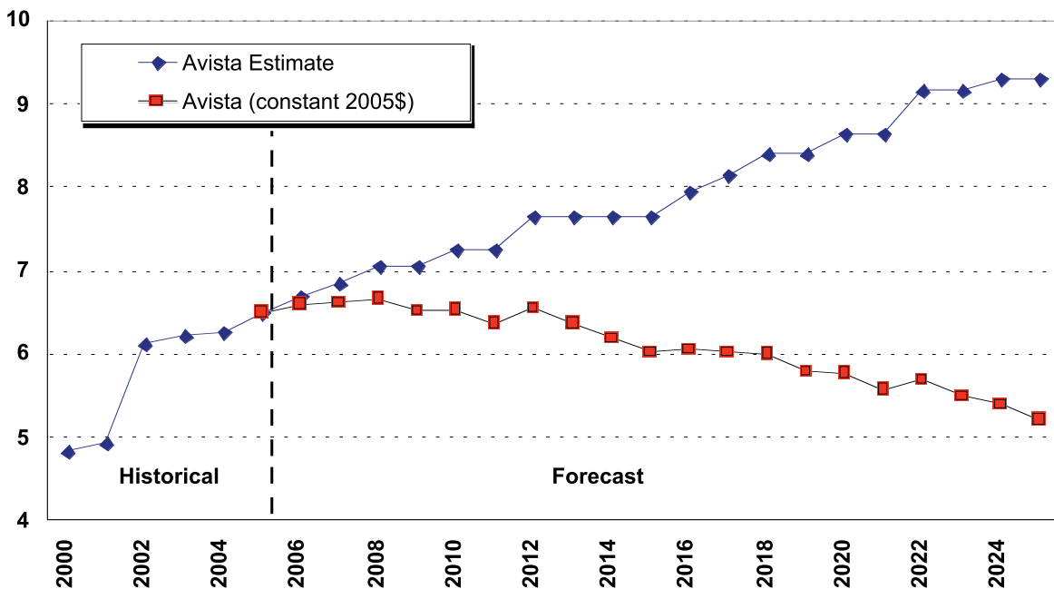
Figure 1.7: Residential Retail Rate Projection for Retail Load Forecast (cents/kWh)
