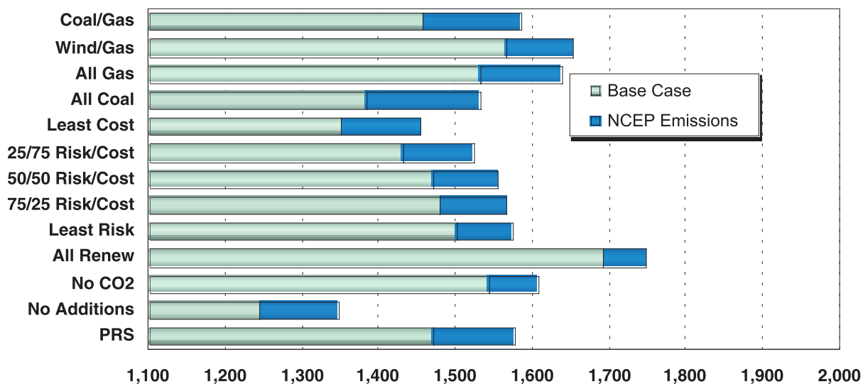
Figure 7.29: 2007-16 Incremental Power Supply Expense NPV ($millions)
