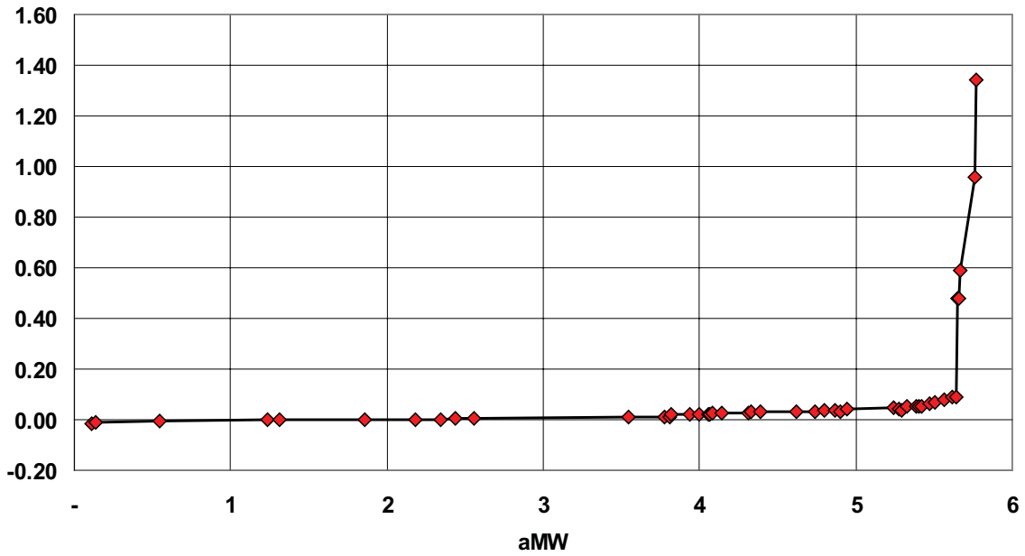
Figure 3.3: Conservation Supply Curve Stacked by Levelized TRC Cost ($)
