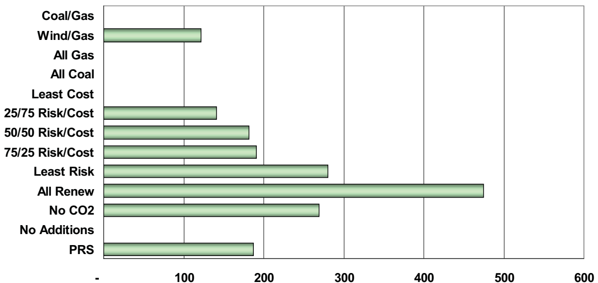
Figure 7.15: Renewable Resource Contribution in 2016 (MW)
