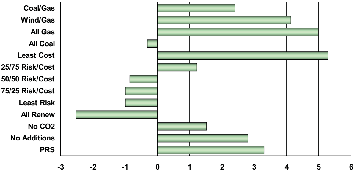
Figure 7.28: Maximum Annual Rate Change from Base Case (%)
