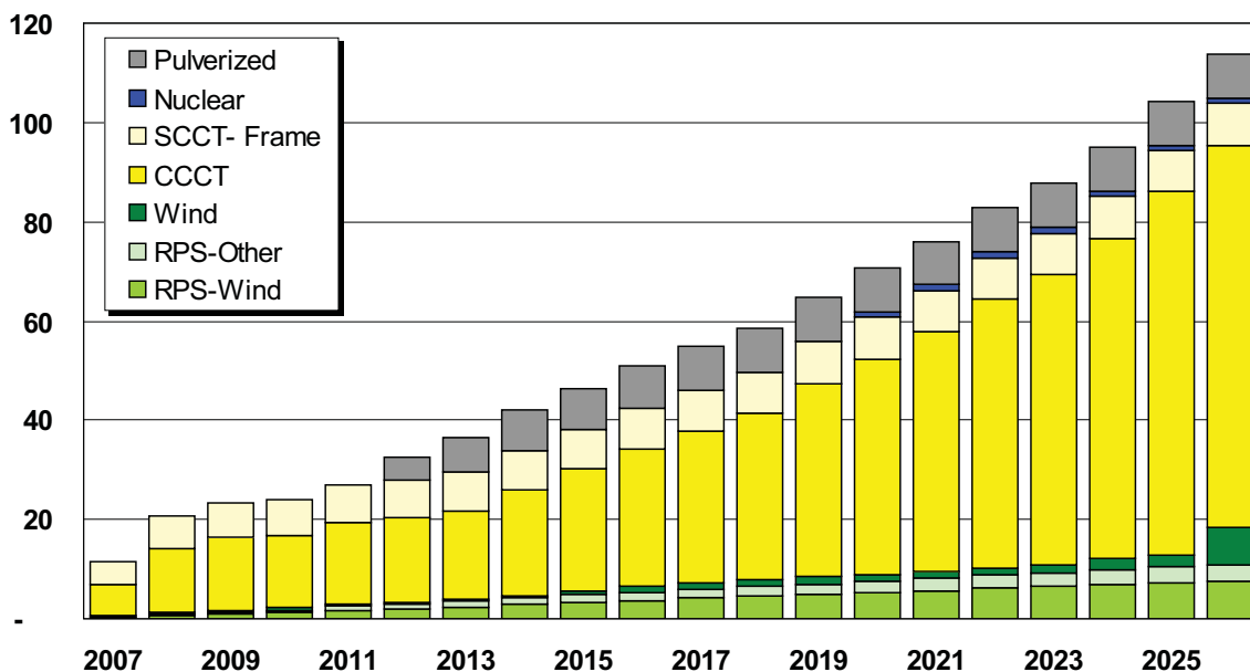
Figure 6.1: Cumulative Western Interconnect Resource Additions (GW)
