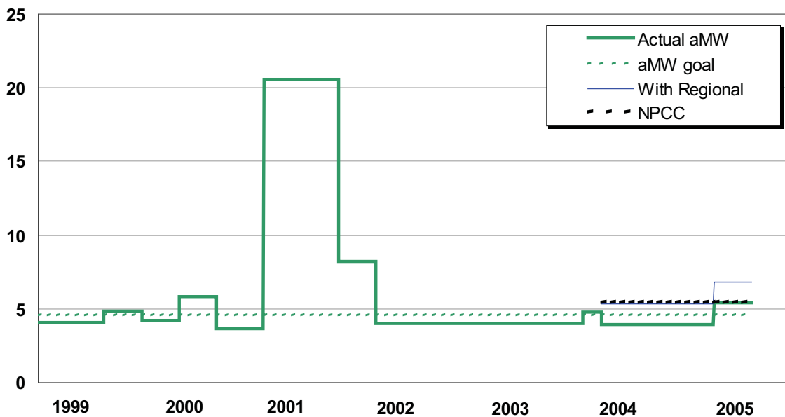
Figure 3.2: Electric Conservation Acquisition Versus Goals (aMW)
