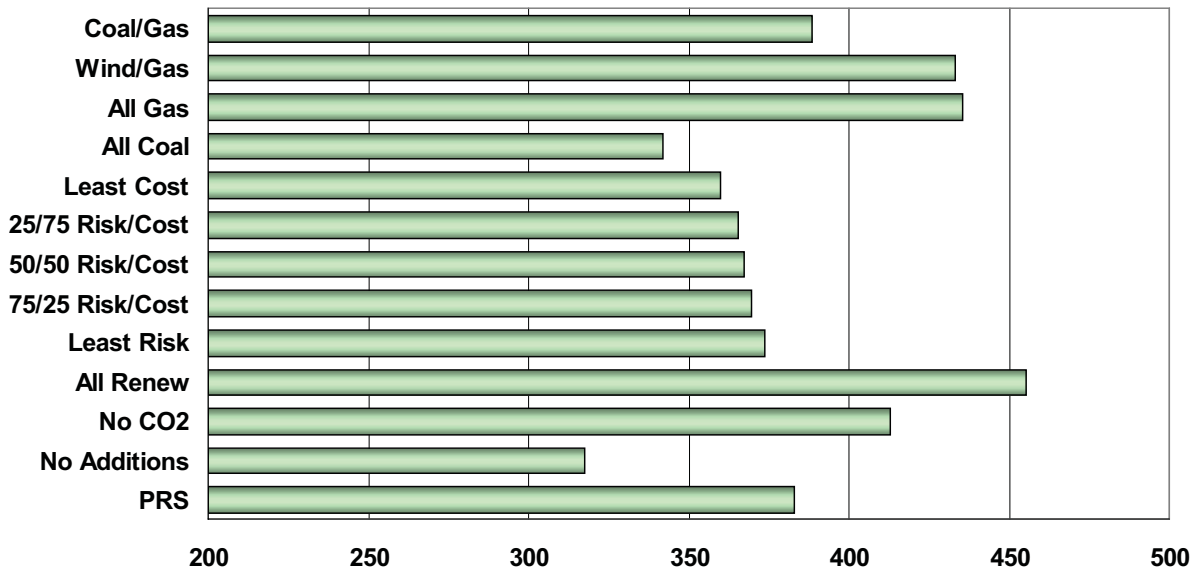
Figure 7.27: 2016 Incremental Power Supply Expense ($millions)
