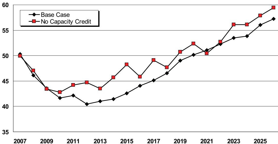
Figure 6.18: Base Case and No Capacity Credit Mid-Columbia Electric Price Forecasts ($/MWh)
