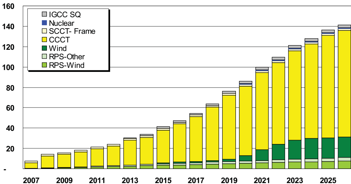
Figure 6.25: Cumulative Resource Selection for the Western Interconnect – SB 342 Carbon Tax (GW)
