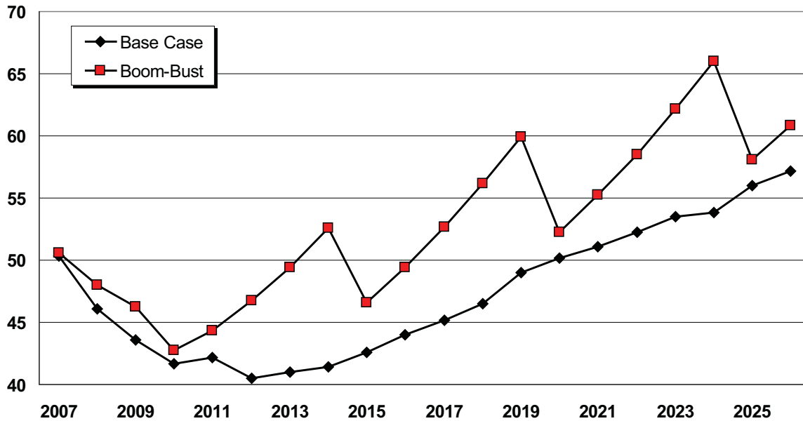
Figure 6.24: Base Case and Boom and Bust Mid-Columbia Electric Price Forecasts ($/MWh)
