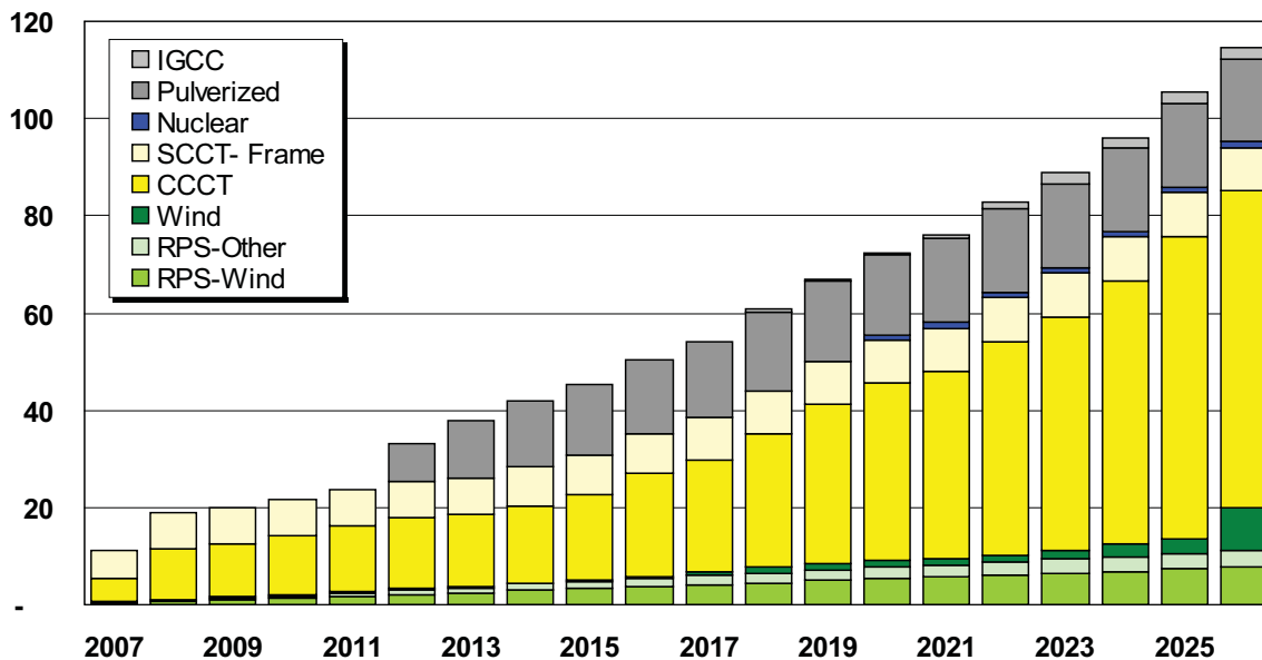
Figure 6.19: Cumulative Resource Selection for the Western Interconnect – 30% Lower Transmission Capital Cost (GW)
