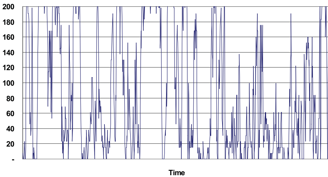
Figure 5.13: Stochastic Wind Model With Serial Correlation (aMW)
