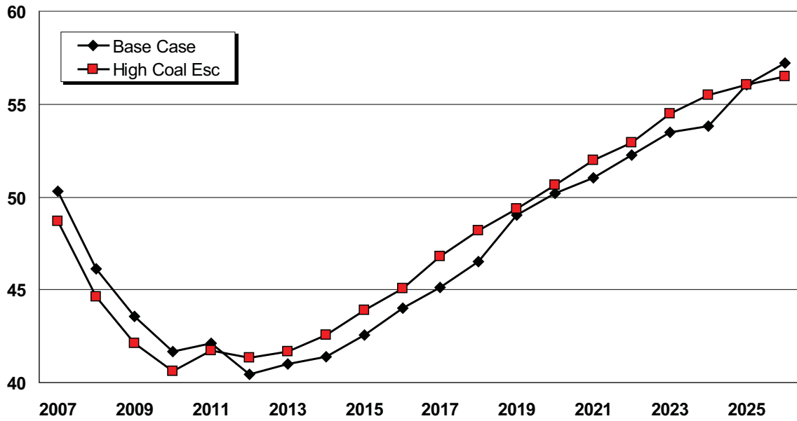
Figure 6.16: Base Case and High Coal Price Escalation Mid-Columbia Electric Price Forecasts ($/MWh)
