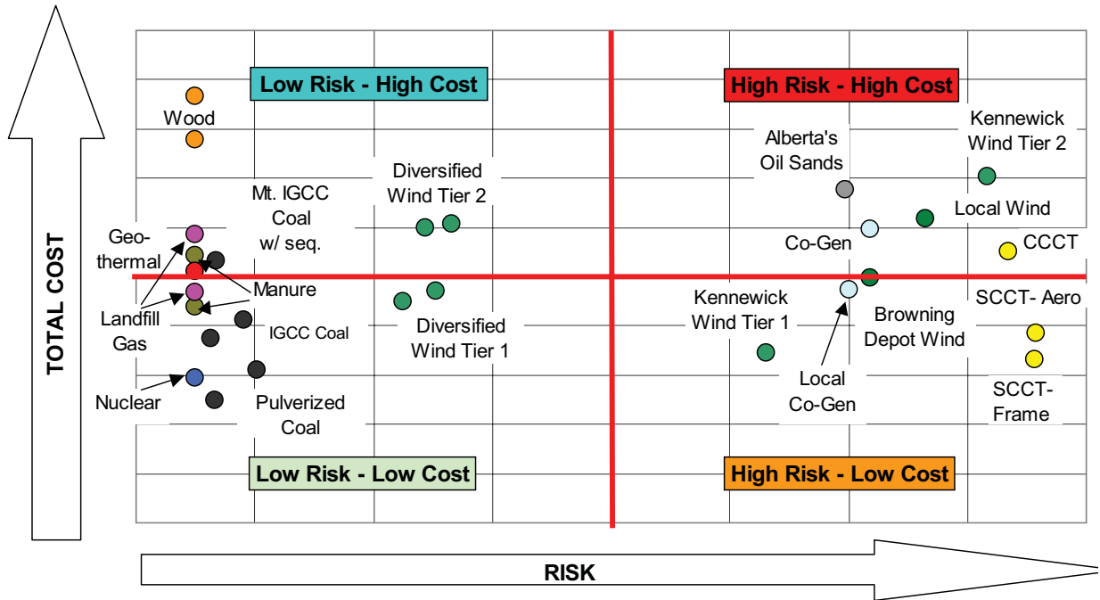
Figure 6.9: Resource Cost and Resource Risk Comparison
