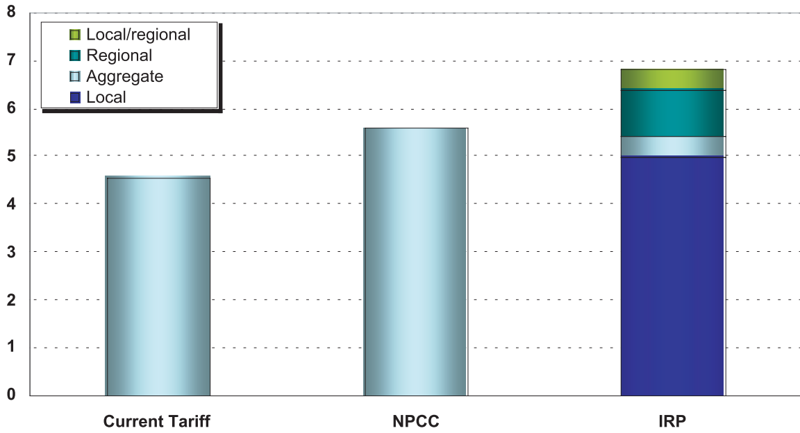
Figure 3.7: Aggregate Conservation Goal Comparison (aMW)
