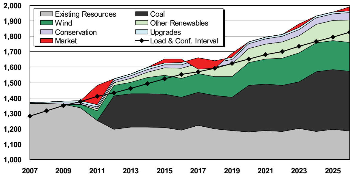
Figure 7.33: Preferred Resource Strategy—Energy (aMW)
