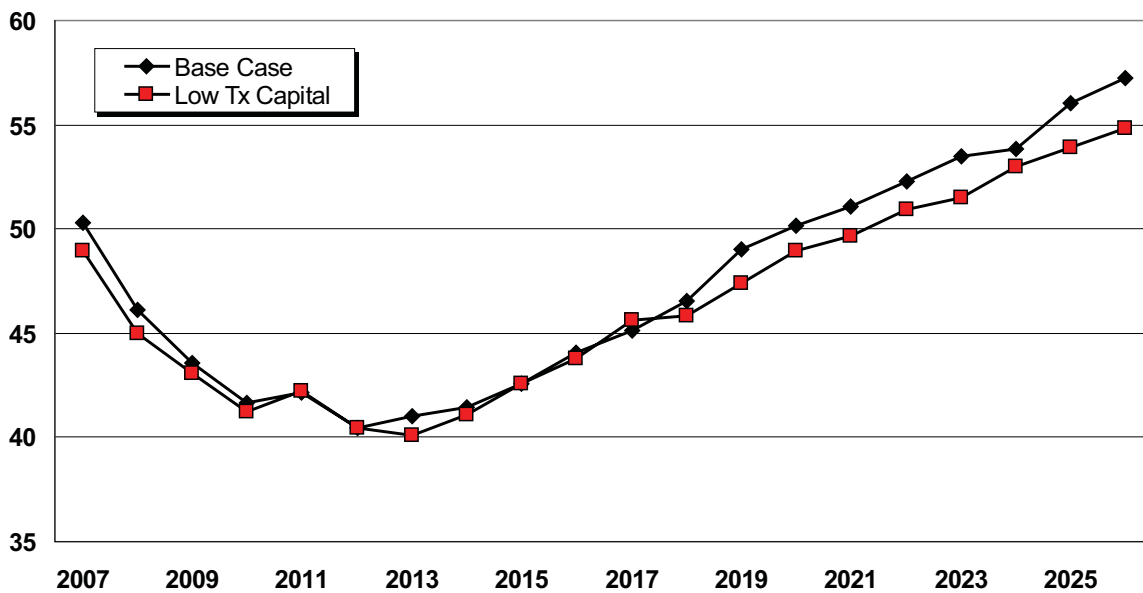
Figure 6.20: Base Case and 30% Lower Transmission Capital Cost Mid-Columbia Electric Price Forecasts ($/MWh)
