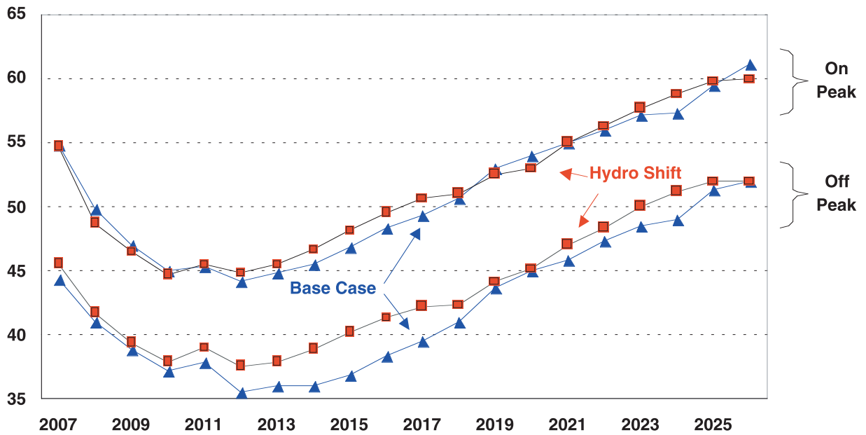
Figure 6.22: Mid-Columbia On & Off Peak Price Comparison For The Hydro Shift ($/MWh)
