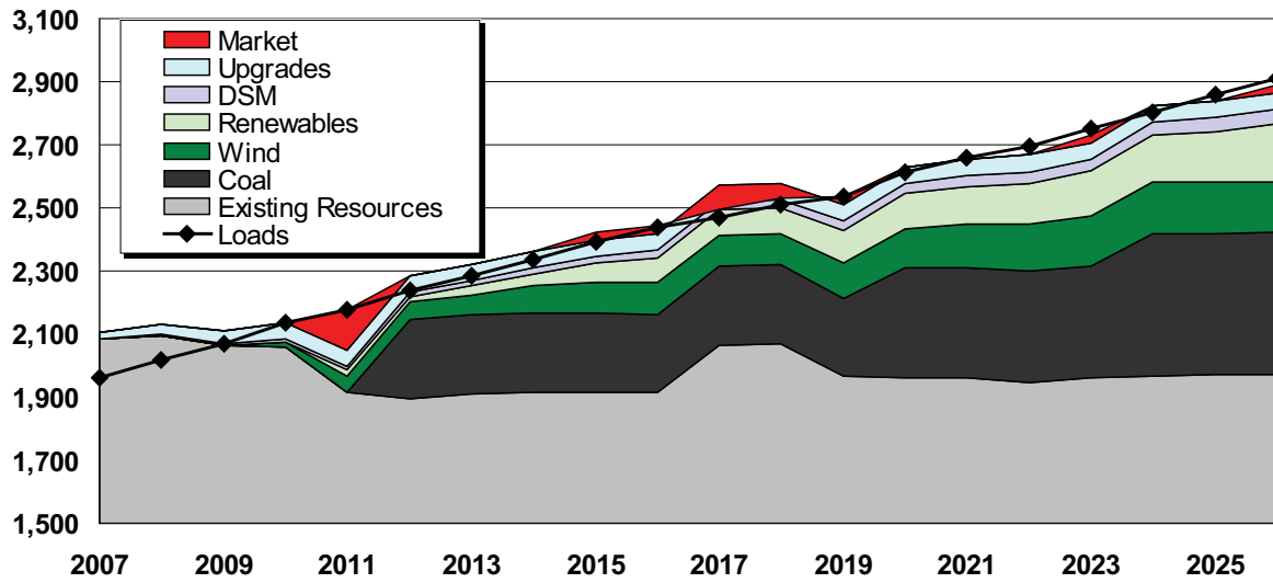
Figure 7.35: Preferred Resource Strategy—Capacity (MW) 9
