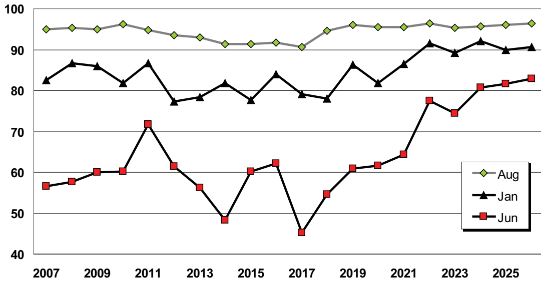
Figure 5.8: Mid-Columbia Electricity and Malin Natural Gas Price Correlations (%)
