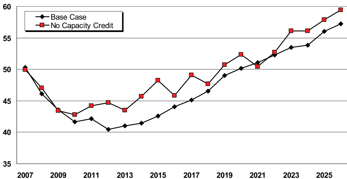
Figure 6.32: Base Case Mid-Columbia Price Forecast and Avoided Costs Comparison ($/MWh)
