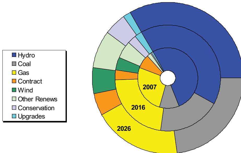
Figure 7.36: Company Resource Mixes (% of Capacity) 2007, 2016, and 2026 10
