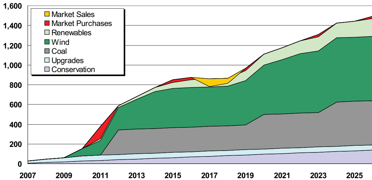
Figure 7.14: Preferred Resource Strategy Build (MW)
