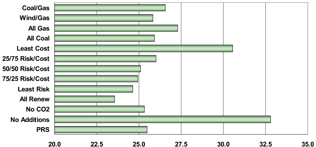
Figure 7.20: 2007-16 Portfolio Risk Comparison-95th Percentile Difference From Mean Value (%)
