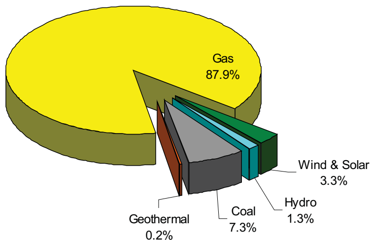
Figure 5.6: New Resources Under Construction (MW)
