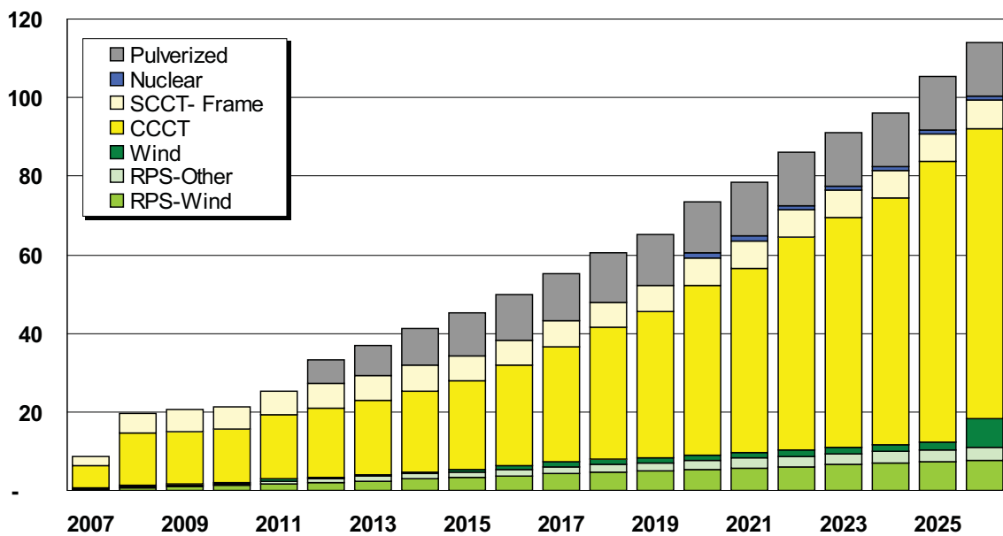
Figure 6.15: Cumulative Resource Selection for the Western Interconnect- High Coal Price Escalation (GW)
