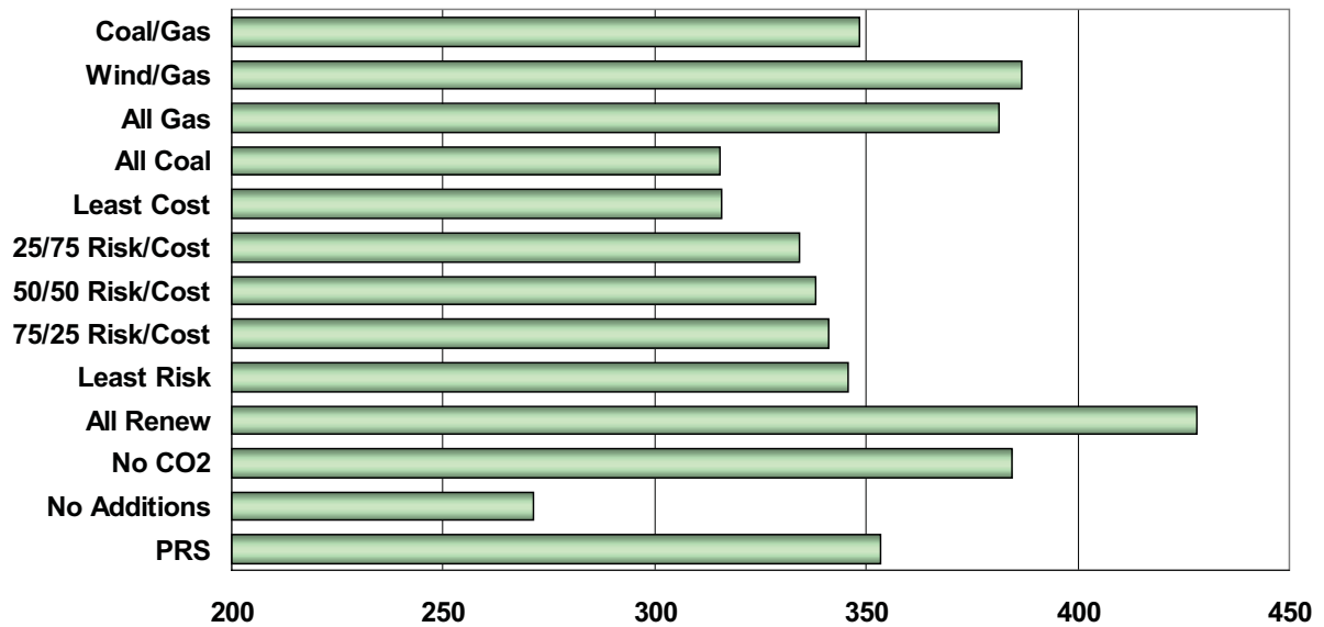
Figure 7.22: 2016 Incremental Power Supply Expense ($millions)
