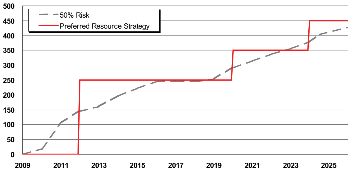
Figure 7.3: Preferred Resource Strategy Coal Build vs. LP Module Build (MW)
