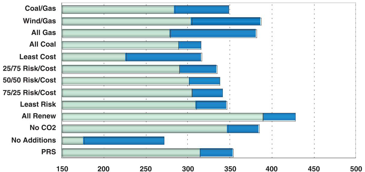
Figure 7.26: 2016 Incremental Power Supply Expense—Low Gas ($millions)
