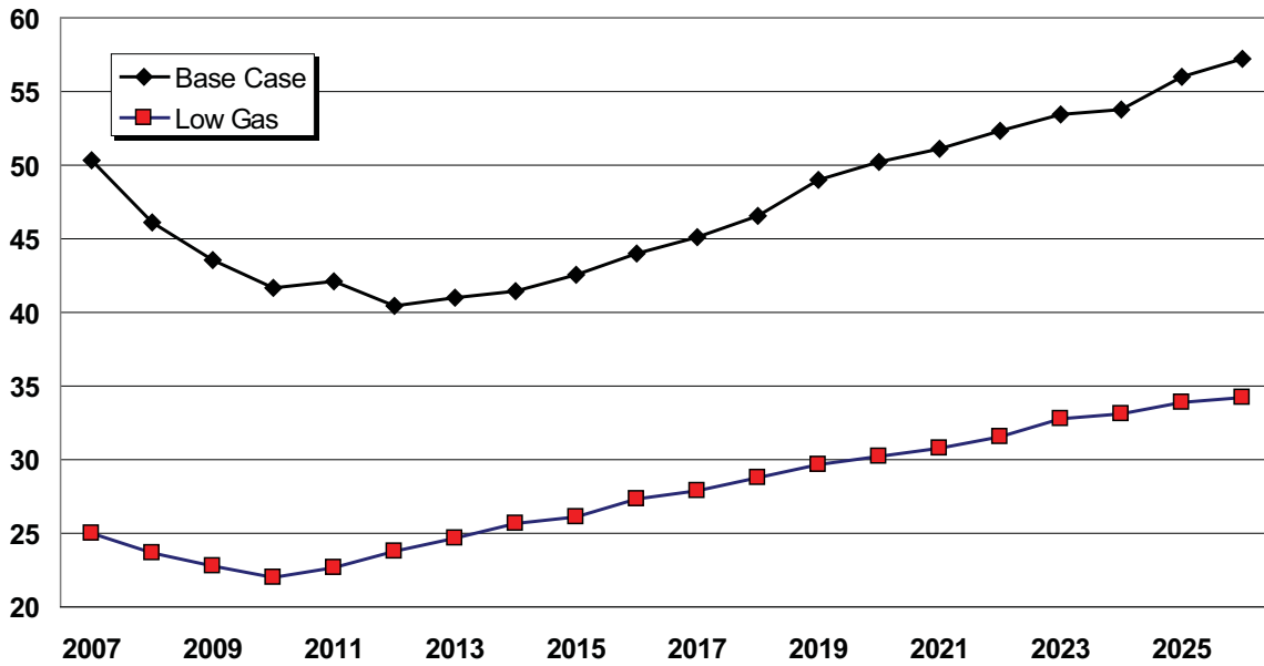
Figure 6.13: Base Case and Low Gas Mid-Columbia Electric Price Forecasts ($/MWh)
