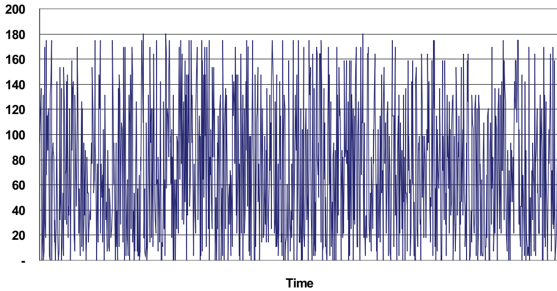
Figure 5.12: Stochastic Wind Model Absent Serial Correlation (aMW)
