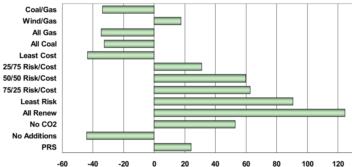
Figure 7.31: 2007-16 Power Supply Expense NPV Change ($millions)
