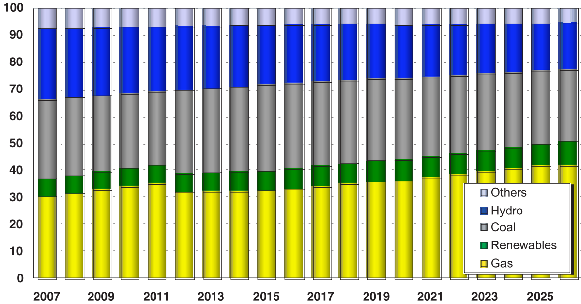
Figure 6.5: Western Interconnect Resource Contribution (%)
