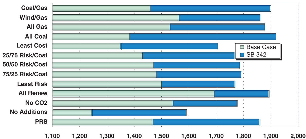
Figure 7.30: 2007-16 Incremental Power Supply Expense NPV ($millions)
